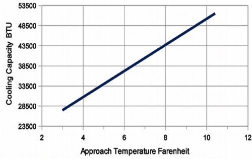
S-4 Evaporator Performance Data US
