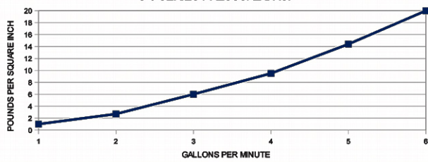
S-5 SERIES PRESSURE DROP
