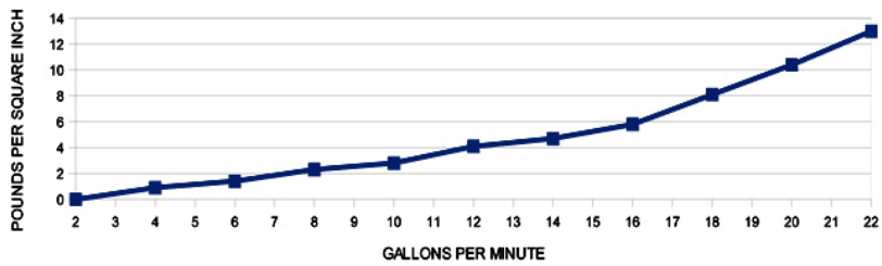
S-6TV PARALLEL PRESSURE DROP
